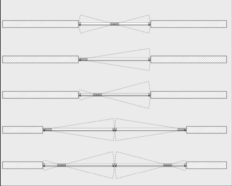
Pivot Doors Opening Options
