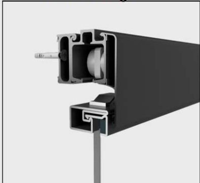
Wall mounted sliding rail
