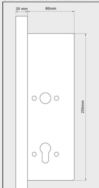
Standard lock-cassette dimensions
